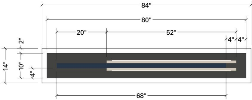
2 PLAN
